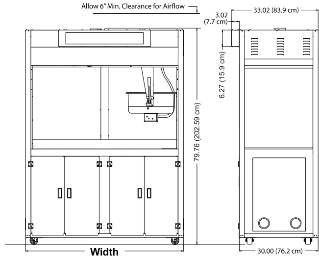
60" Cabinet shown for dimension reference only.
